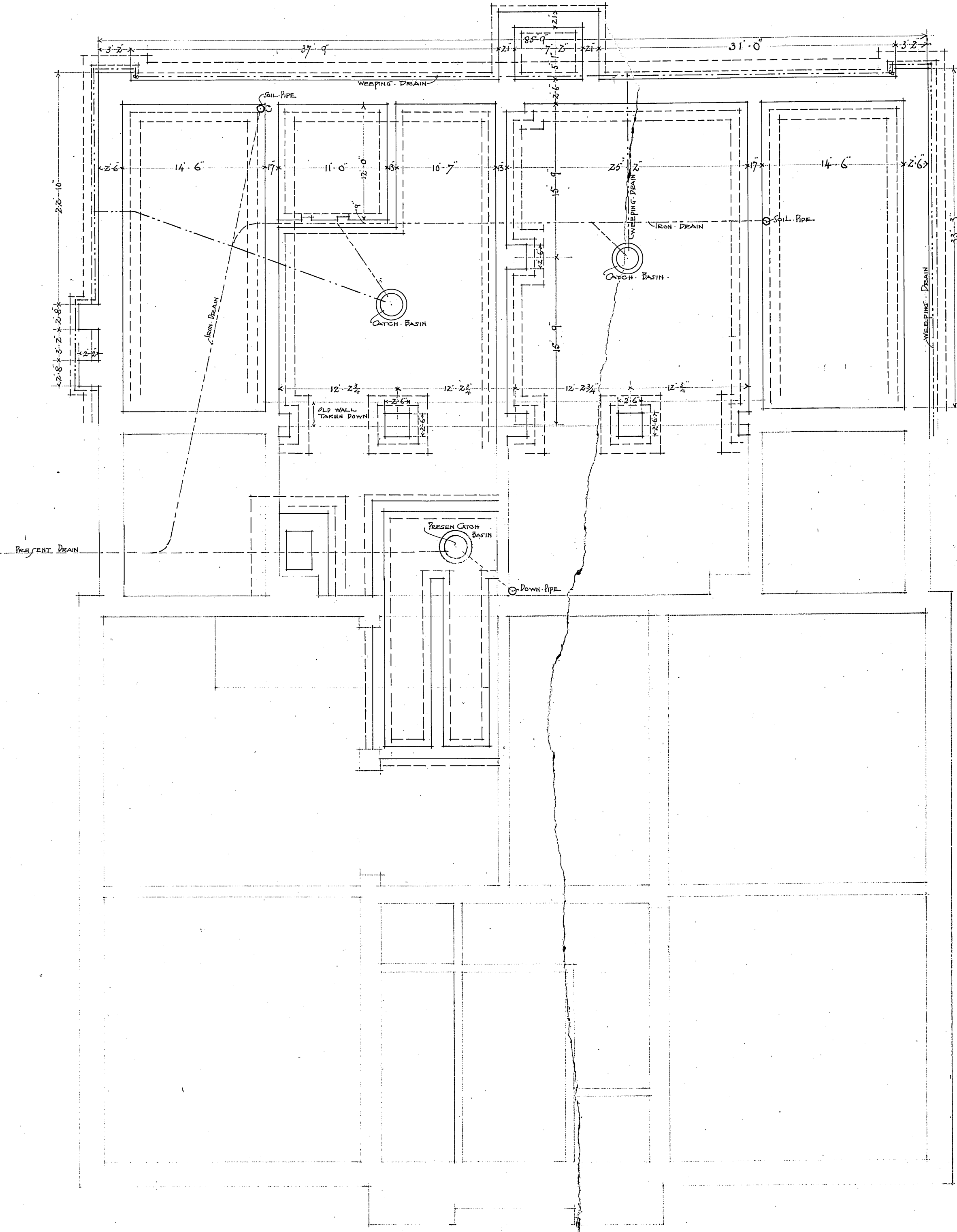
FOUNDATION PLAN
